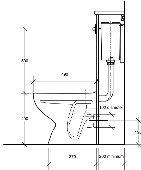
Ifö Cera ES4 Back to Wall
